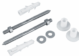
RAG BOLTS FOR WASH BASIN Catalogue No. RB-WB 80002-12
